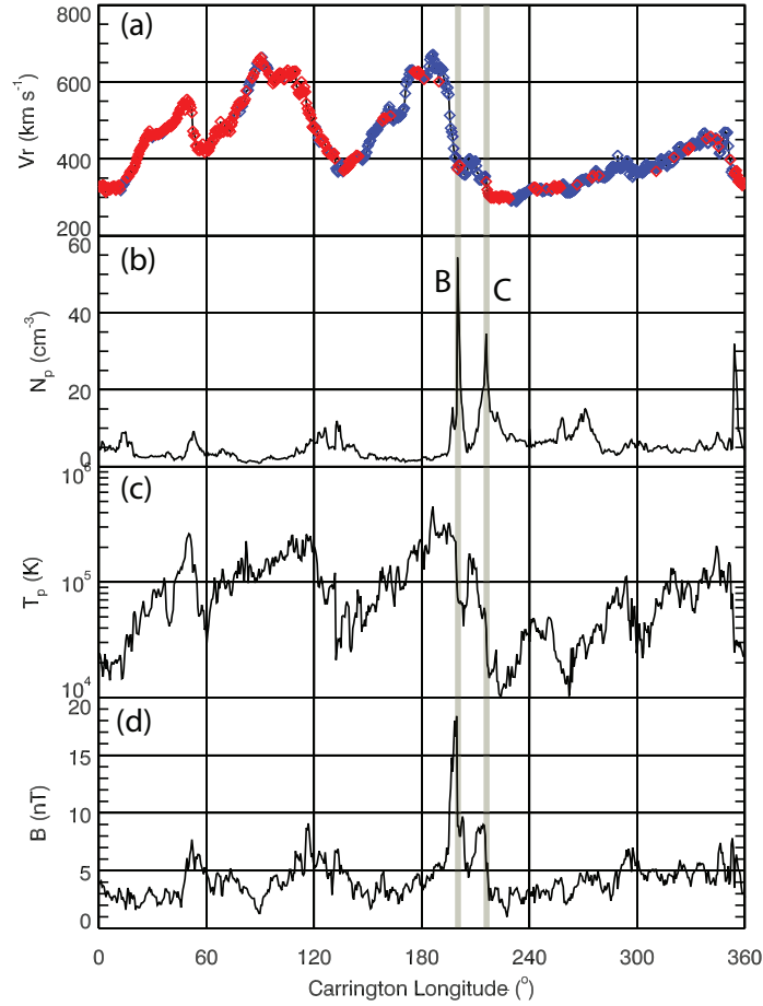
Figure 9. (a) Solar wind speed; (b) number density; (c) proton temperature; and (d) magnetic field strength as a function of Carrington longitude (at 1 AU) for Carrington rotation 2060. Two density enhancements are labeled ‘B’ and ‘C’ and discussed in more detail in the text.
