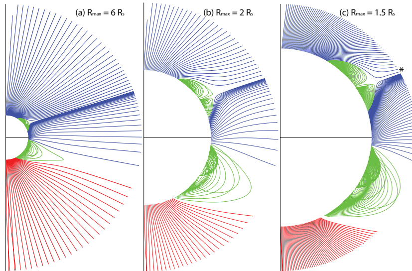
Figure 10. A selection of magnetic field lines for CR 2060 at a longitude of 215^\circ are shown at successively smaller scales: (a) R_{\max} = 6R_\odot ; (b) R_{\max} = 2R_\odot ; and (c) R_{\max} = 1.5R_\odot . For (a) and (b), 185 field lines equally separated in latitude were drawn. For (c), 370 field lines were drawn. The apparently intersecting field lines is a projection effect due to field lines having different ending longitudes.
