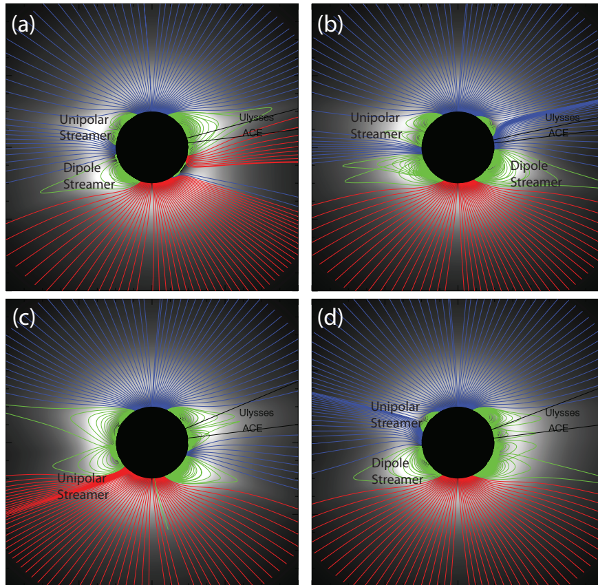
Figure 1. A selection of meridional slices from a global MHD simulation of CR 2060, which occurred between 14 August 2007 and 10 September 2007. Grey-scale images are Simulated polarized brightness ( pB ) images and the colored lines are magnetic field lines drawn from equally-spaced points in latitude on the solar surface. The field lines have been color-coded so that blue/red lines are field lines that open into the heliosphere and are inwardly/outwardly directed, while green field lines connect back to the Sun at both ends, i.e. , they are closed field lines.
