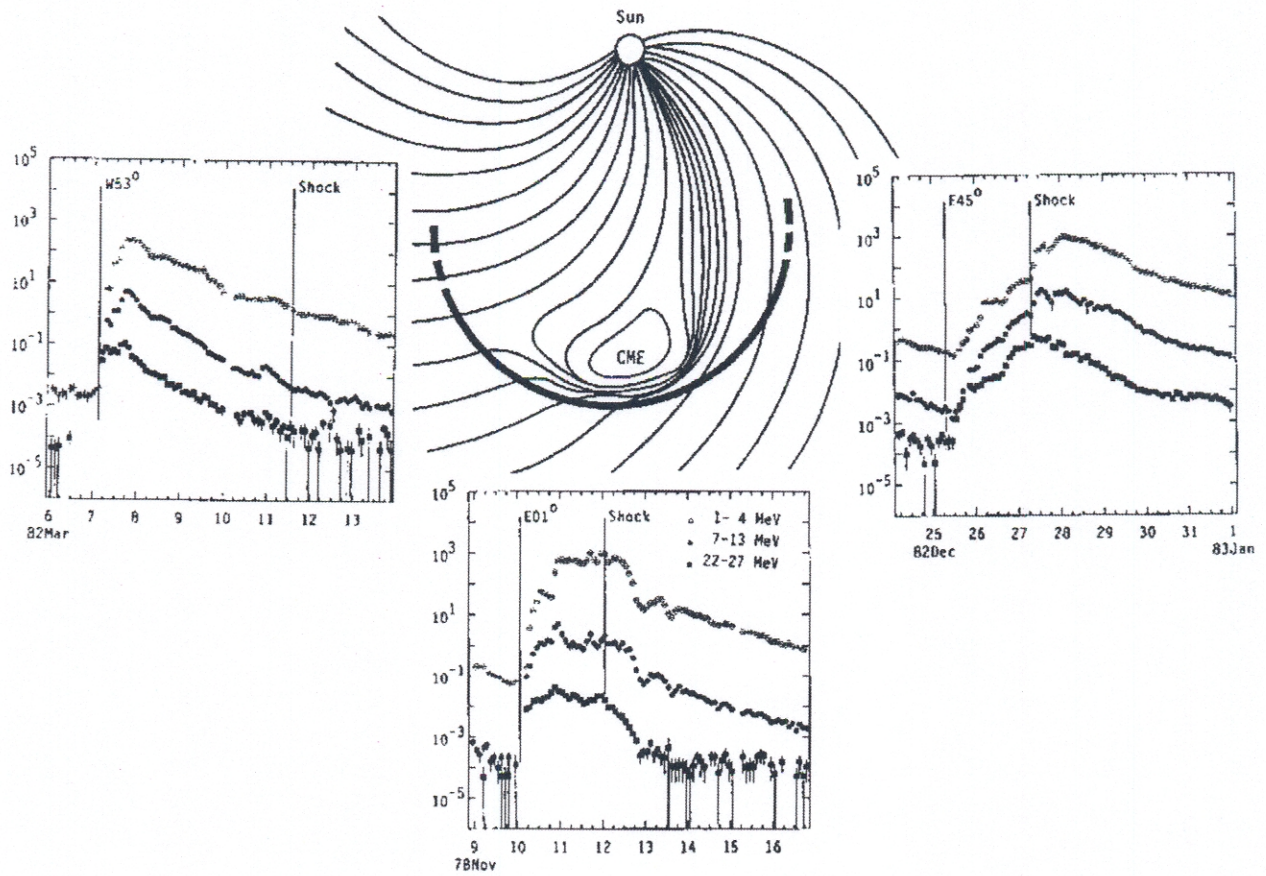
Figure 1. Illustration from Reames (1999) of the geometrical organization of observed SEP event time profiles to the CME shock driver and interplanetary shock source. The strongest source region is considered to be located at the nose or leading portion of the shock. The SEPs travel to first order along field lines connecting the shock source and the observer, as the shock moves outward.
