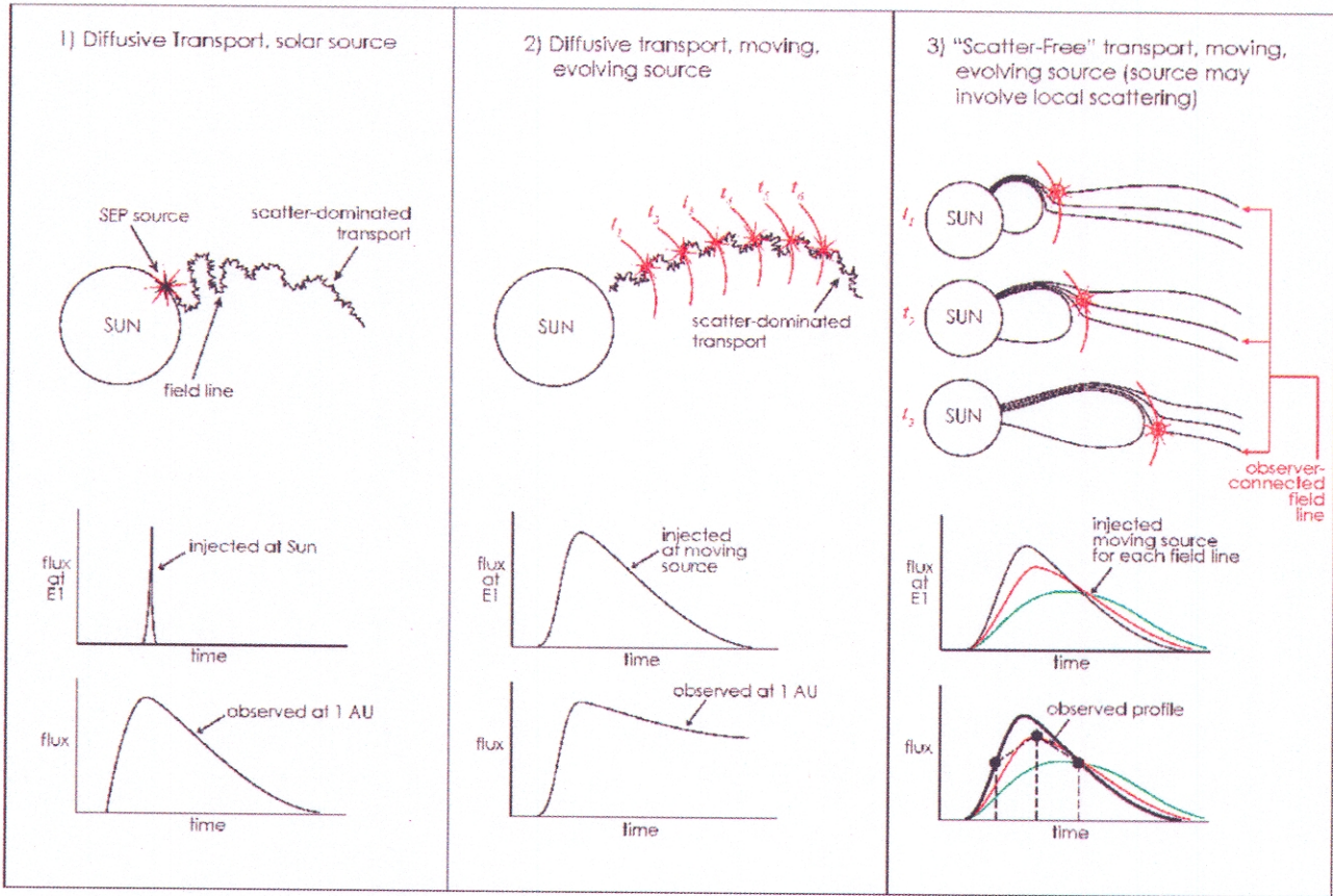
Figure 4. Illustration of various views of SEP event sources and transport. The left-hand column illustrates a source on the Sun followed by diffusive propagation through fluctuating magnetic fields. The center column illustrates a moving shock source with diffusive propagation. The right column illustrates the concept adopted in our model, which initially involves sampling the events on a sequence of connected field lines to get the observed profile, and scatter-free motion outside of the shock source on the field lines.
