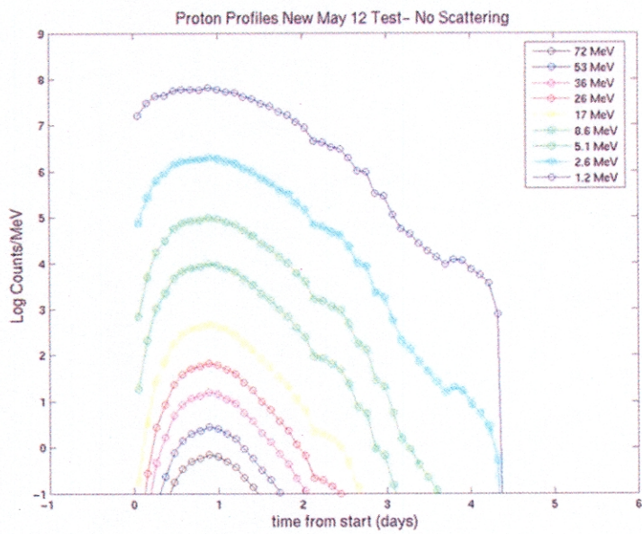
Figure 5. Modeled SEP event for the May 12, 1997 cone model event simulation based on a simplified shock source parameterization and scatter-free transport. No attempt has been made to model the ESP peak at shock arrival or the effects of CME ejecta fields which are not included in the cone model simulation.
