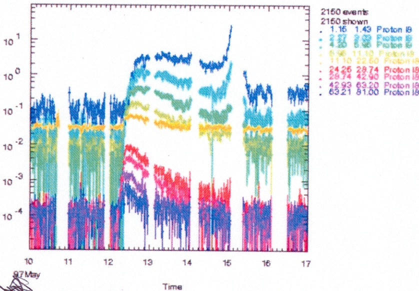
Figure 3. IMP observations of the SEP event associated with the May 12, 1997 halo CME (courtesy of A.J. Tylka).
