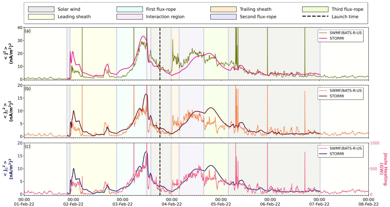
Figure 8. The panels illustrate the correlation between the outcomes derived from SWMF/BATS-R-US and STORMI. Panel (a) and (b) demonstrate the temporal profile similarity of \langle J^2 \rangle and \langle J_{\parallel}^2 \rangle , respectively. In panel (c), the Ionospheric Joule heating from SWMF/BATS-R-US and \langle J_{\parallel}^2 \rangle are plotted side by side, using parallel and color-coded y-axis to visually highlight the qualitative resemblance.
