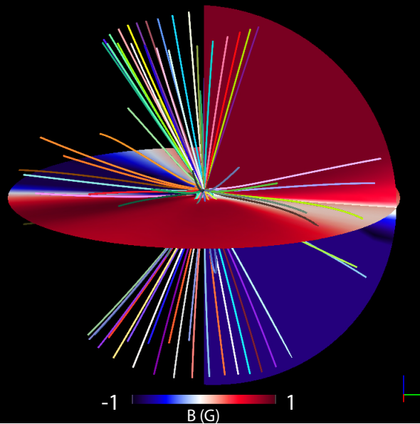
(c) Whole Sun Month: Heliosphere
